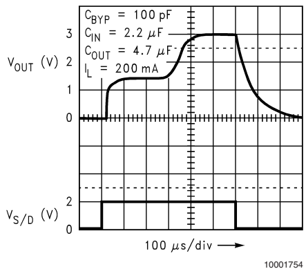
Turn-On Time (LP2988)
