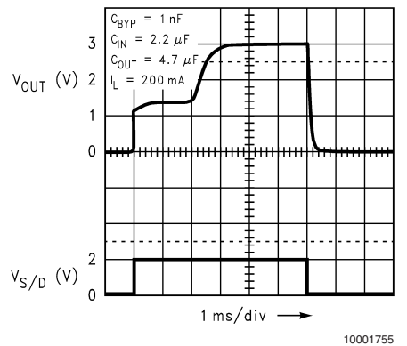
Turn-On Time (LP2988)
