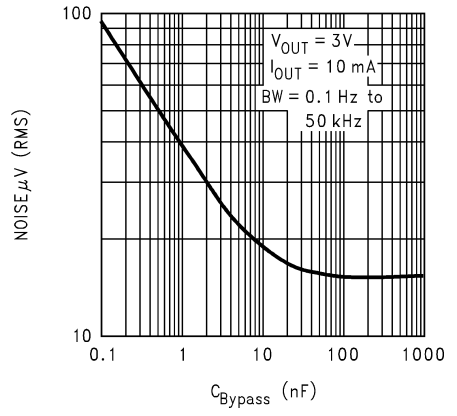
Output Noise Voltage (LP2988)
